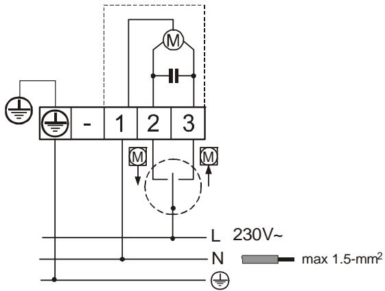
VA-7700-xx03 Floating models, 230 VAC supply
