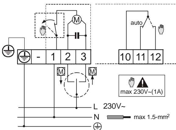
VA-7740-xx03 Floating models, 230 VAC supply
