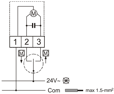
VA-7700-xx01 Floating models, 24 VAC supply
