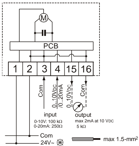
VA-7706-xx01 Proportional models, 24 VAC supply
