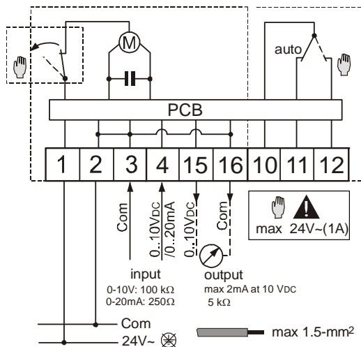
VA-7746-xx01 Proportional models, 24 VAC supply
