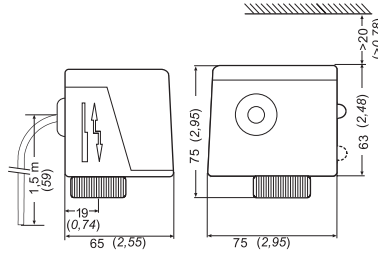
Dimensions in mm (inches)
