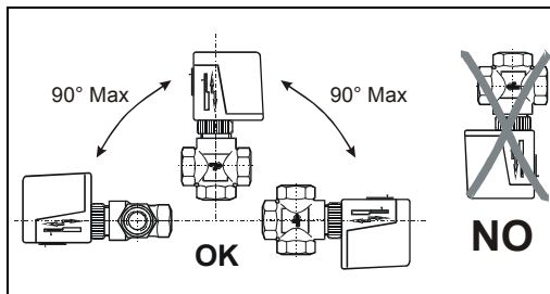
Mounting Positions
