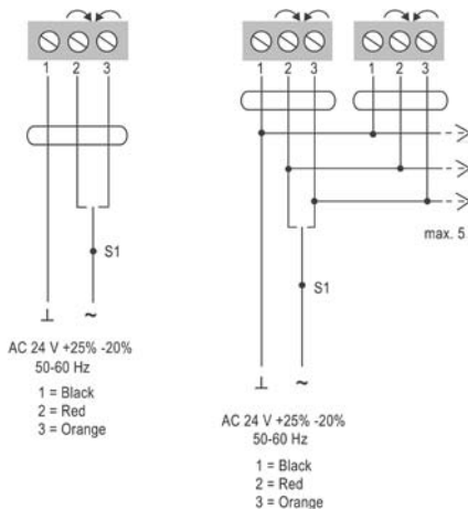
Wiring Diagram
