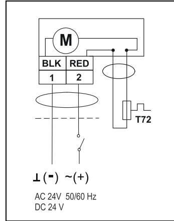
Figure 8: S9208-BGC-33A ON/OFF Control Wiring Diagram
