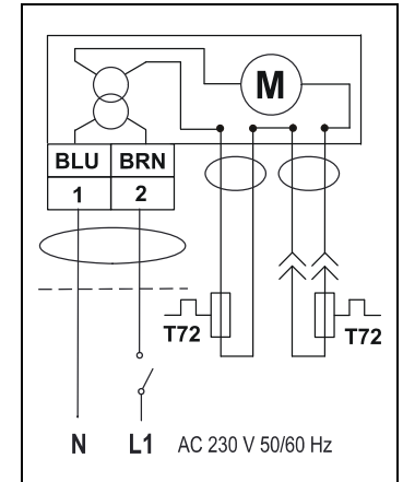
Figure 13: S9208-BDC-33C ON/OFF Control Wiring Diagram
