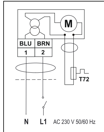
Figure 12: S9208-BDC-33A ON/OFF Control Wiring Diagram
