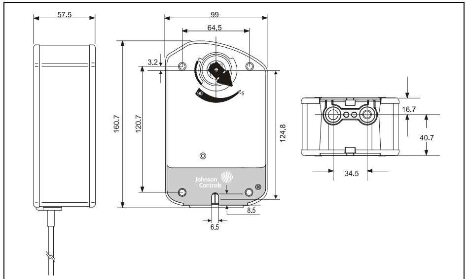
Figure 1: Dimensions in mm
