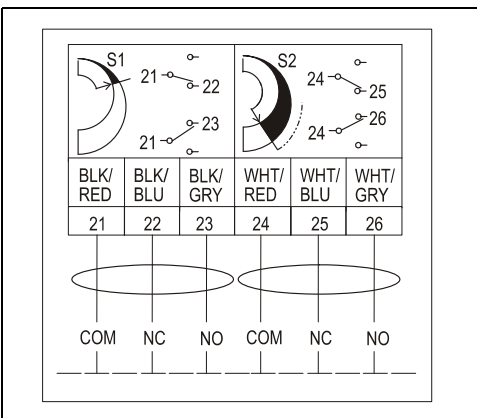
Figure 14: Auxiliary Switch Wiring Diagram
