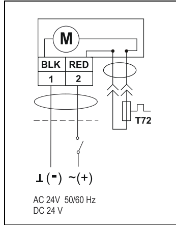
Figure 7: S9208-BGC-33B ON/OFF Control Wiring Diagram
