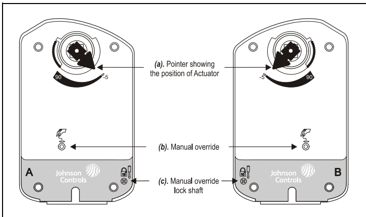
Figure 2: Side A and Side B of Actuator
