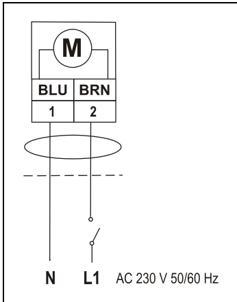
Figure 10: S9208-BDC-33 ON/OFF Control Wiring Diagram
