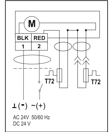
Figure 9: S9208-BGC-33C ON/OFF Control Wiring Diagram
