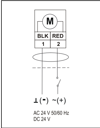
Figure 6: S9208-BGC-33 ON/OFF Control Wiring Diagram
