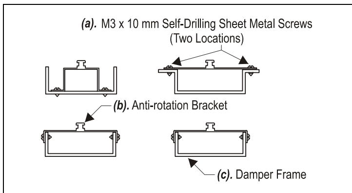
Figure 3: Fitting the Anti-rotation Bracket on the Damper Frame or Duct
