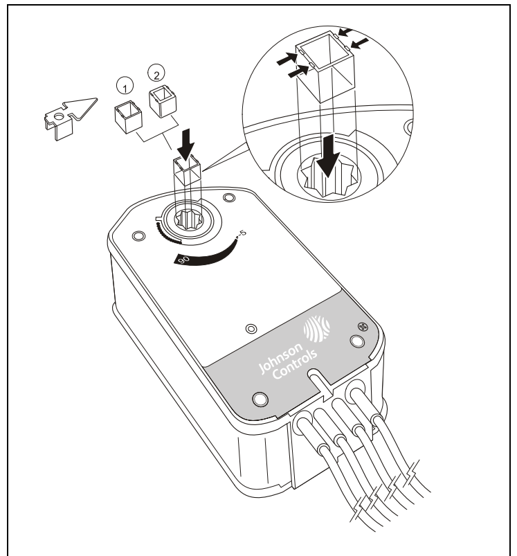
Figure 4: Changing the dimensions of the coupler
