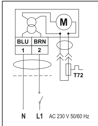
Figure 11: S9208-BDC-33B ON/OFF Control Wiring Diagram
