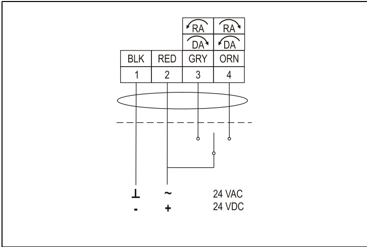
Figure 7: Floating Control, Four Wire M92x0-AGx-1
