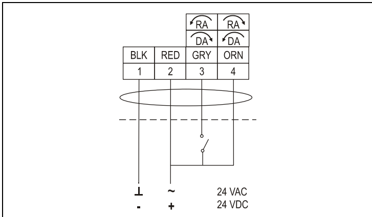
Figure 8: Open / Close, Single Wire Control M92x0-AGx-1
