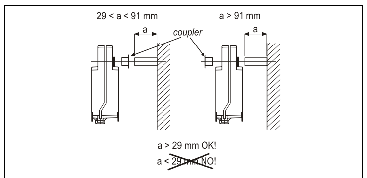
Figure 5: Allowed shaft length
