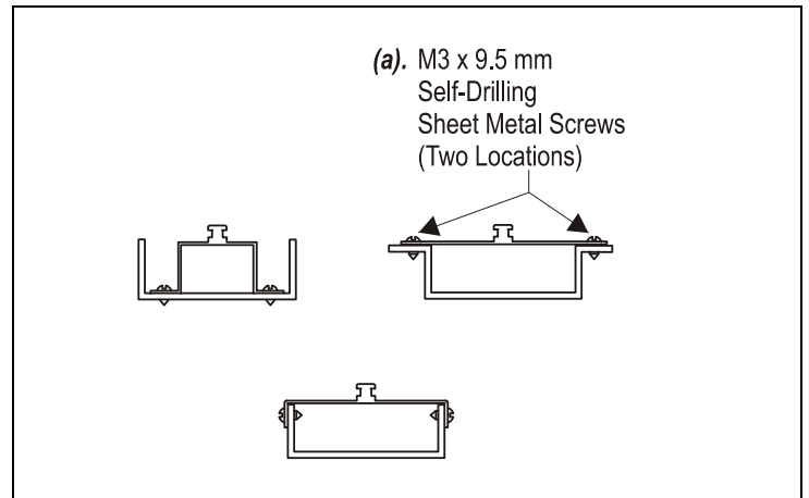
Figure 3: Fitting the Anti-rotation Bracket on the Damper Frame or Duct
