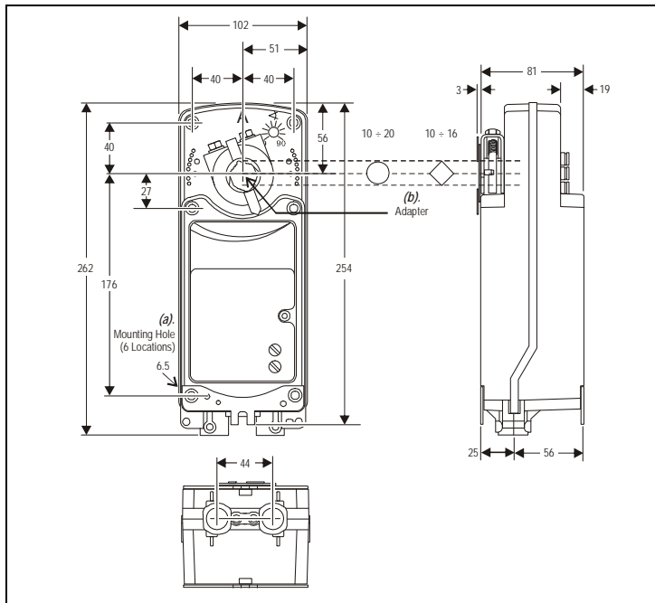
Figure 1: Dimensions in mm
