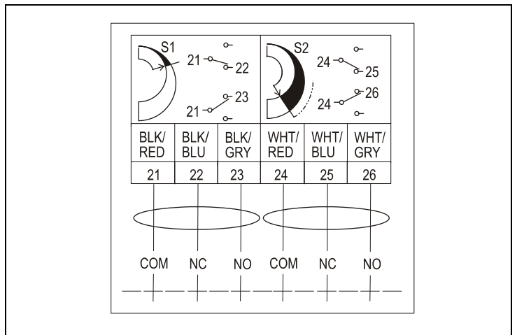
Figure 12: Auxiliary switch wiring diagram
