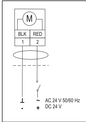
Figure 10: ON/OFF Control M92x0-BGx-1
