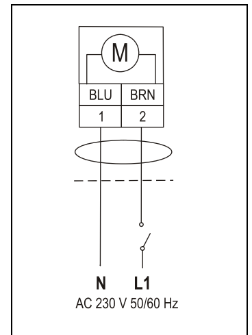
Figure 11: ON/OFF Control M92x0-BDx-1
