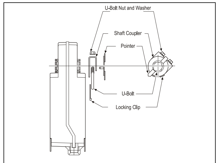
Figure 4: Changing the position of the Coupler
