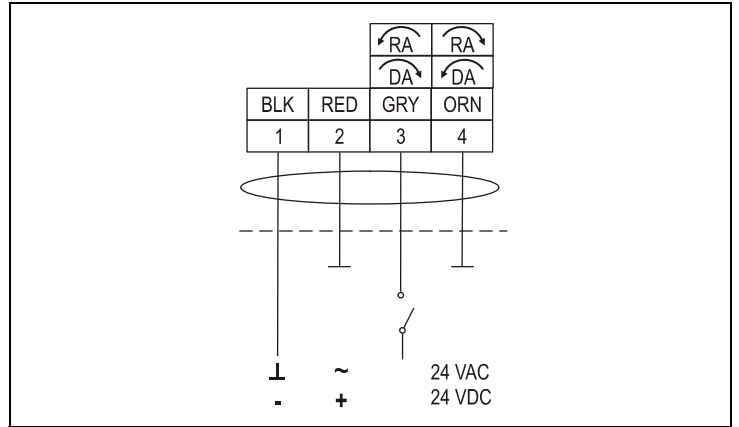
Figure 9: ON/OFF Control, Two Wire M92x0-AGx-1
