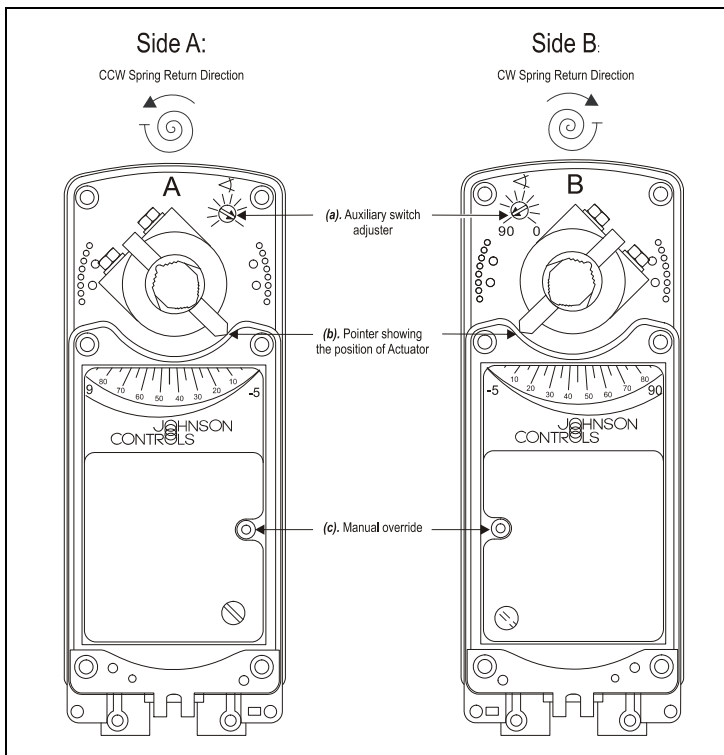
Figure 2: Side A and Side B of Actuator
