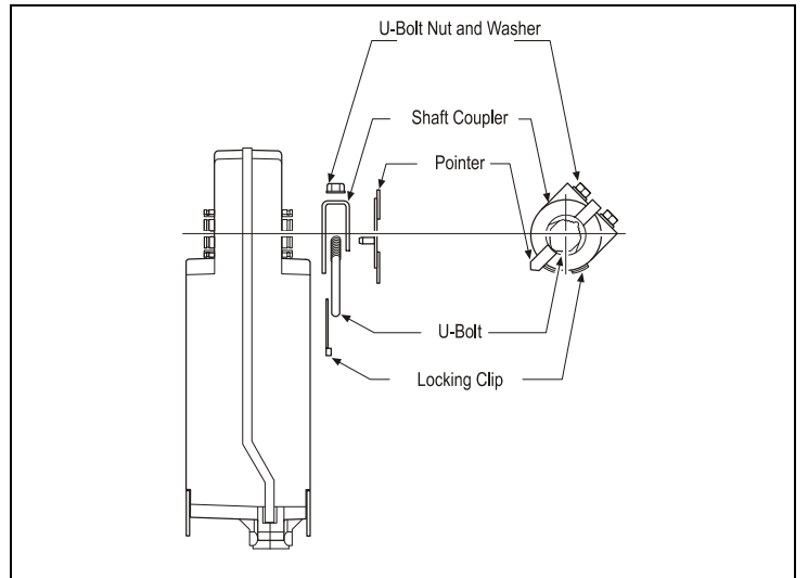
Figure 4: Changing the position of the coupler
