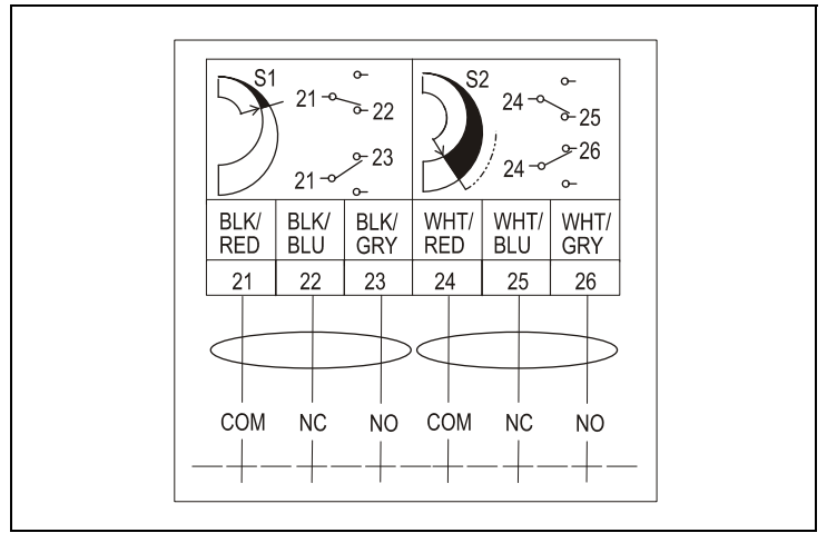
Figure 9: Auxiliary switch Wiring Diagram
