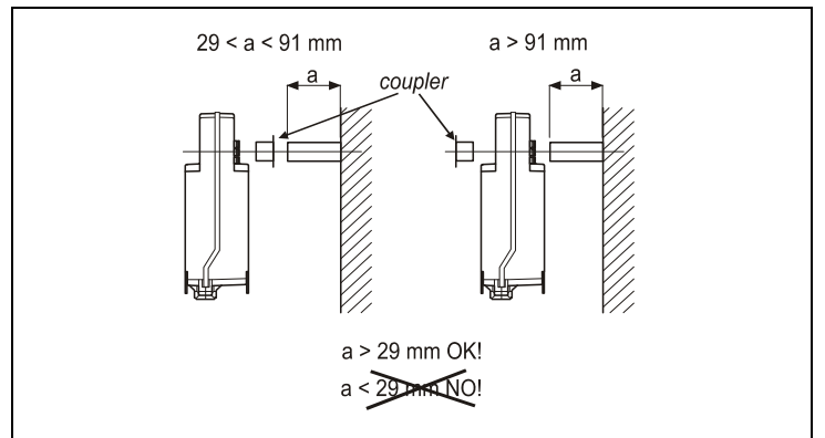
Figure 5: Allowed shaft length
