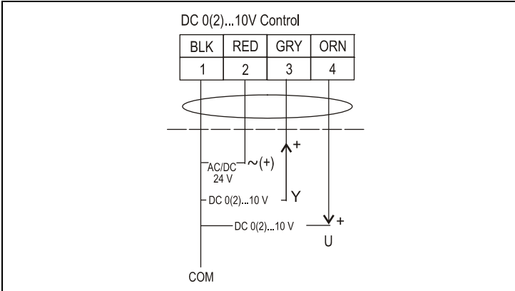
Figure 7: Proportional control 0(2)...10 VDC Wiring Diagram
