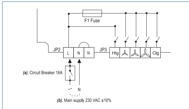
FX03 230 VAC Power Supply
