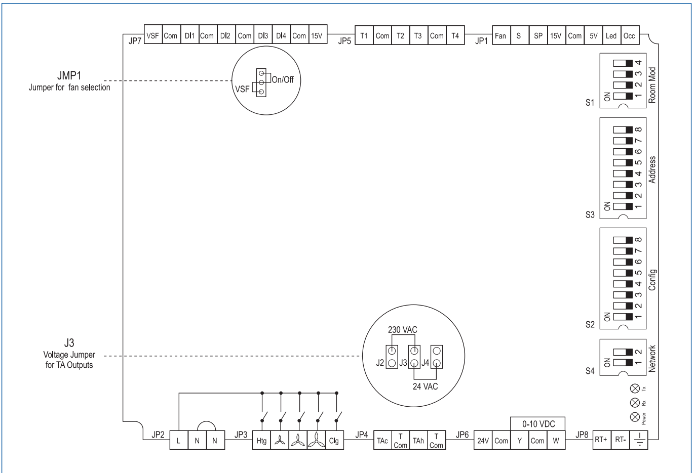
FX03 Jumper Configuration
