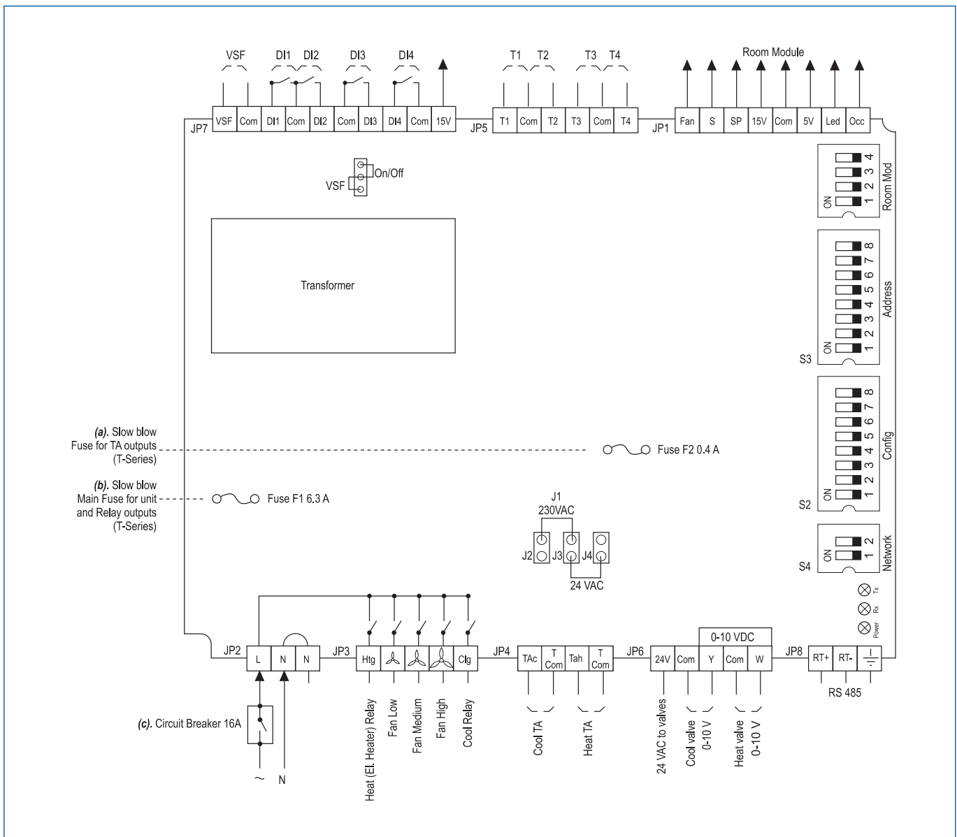
FX03 Wiring Diagram
