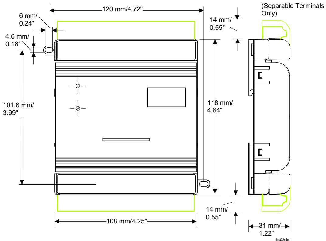
Figure 13: TC-9102 Controller Dimensions
