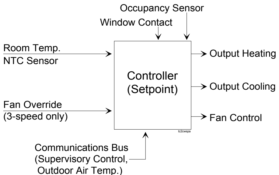
Figure 5: Controller with Integrated Setpoint Adjuster
