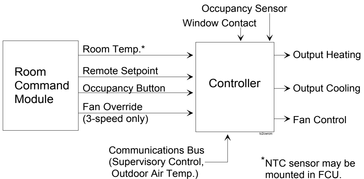
Figure 4: Controller with Room Command Module
