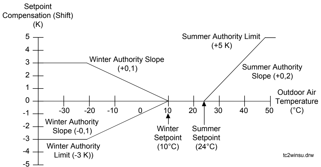
Figure 6: Winter/Summer Compensation
