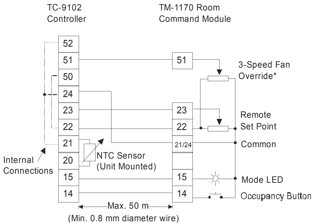
Figure 18: TC-9102 Controller Wiring to Room Command Module with Unit Mounted NTC Sensor
