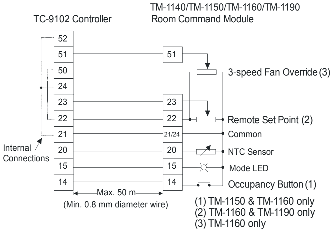
Figure 17: TC-9102 Controller Wiring to Room Command Module with Integral NTC Sensor
