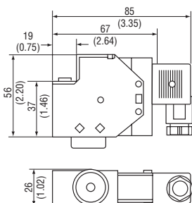
Dimensions in mm (inches)
