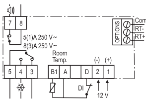
MR42PM12R-A1C Wiring
