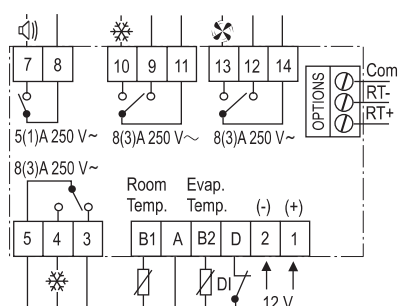
MR44PM12R-A2C Wiring
