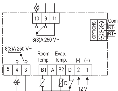
MR43PM12R-2C Wiring
